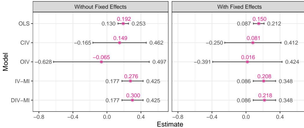
Figure 4: Peer Effect Estimates and Confidence Intervals
