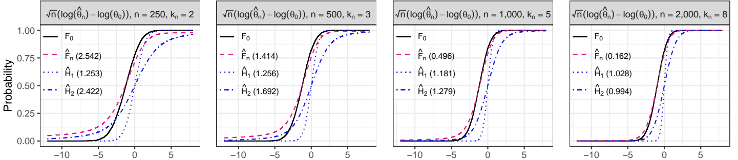
Figure 3: Monte Carlo Simulations: Estimates of asymptotic CDFs (DGPs C and D)
