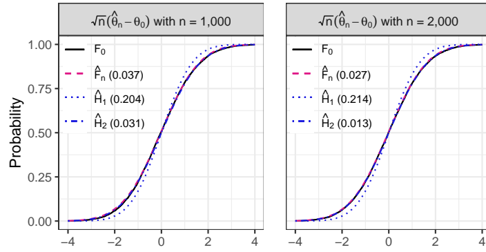
Figure 1: Illustration of the asymptotic CDF estimates
