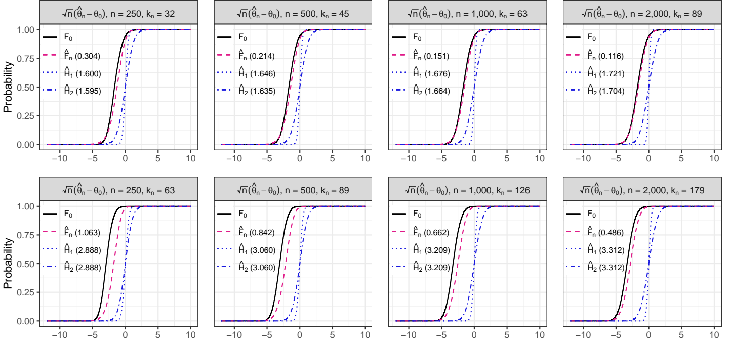
Figure 2: Monte Carlo Simulations: Estimates of asymptotic CDFs (DGPs A and B)
