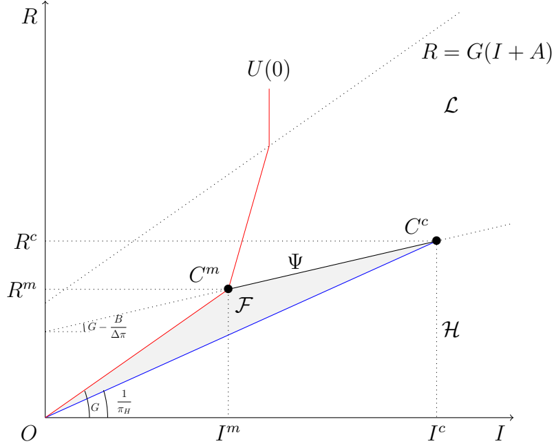
Figure 1: Set \mathcal{F} of aggregate feasible allocations.
