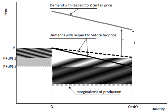
Figure 1b: Ad valorem taxes
