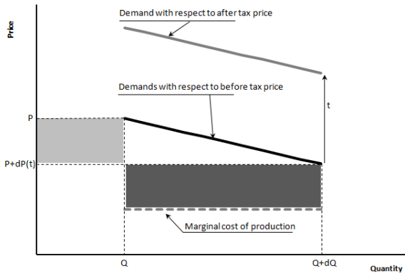
Figure 1a: Per unit taxes
